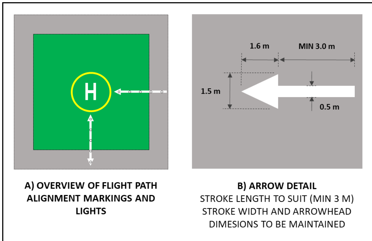
Figure 31: Flight path alignment guidance markings and lights
